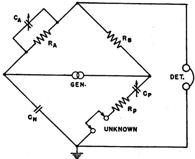
FIGURE 1. Basic circuit of Type 916-A Radio-Frequency Bridge
