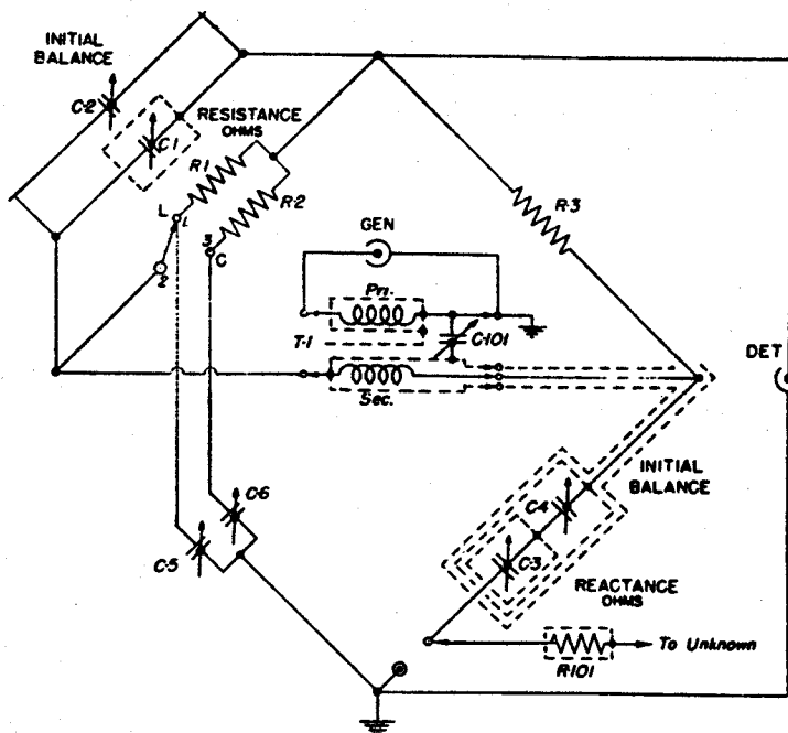
Figure 8. Complete Wiring Diagram for Radio-Frequency Bridge.
